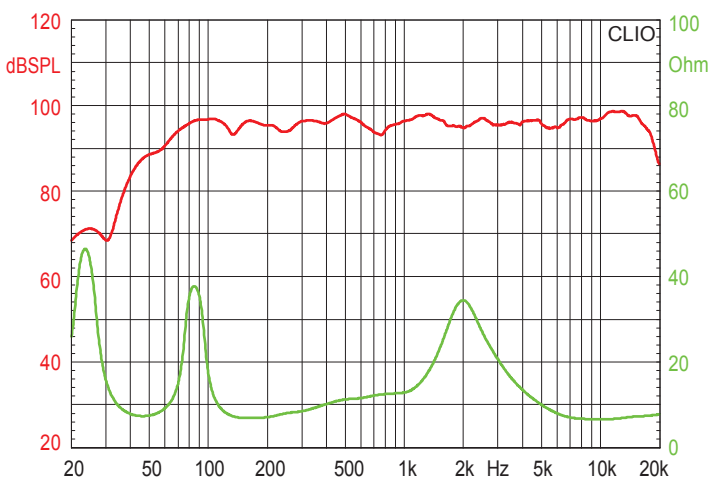
MLS-Frequency Response & Impedance- 1/3octave 1W/1m 2PI(half space)
